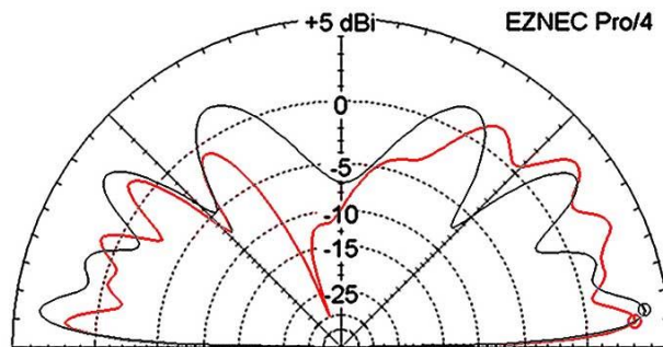
Figure 7: Comparative elevation radiation patterns and gains, Vent Antenna (black), J-pole (red)
