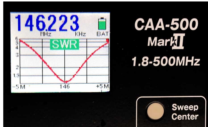
Figure 6: SWR and Bandwidth on a Comet CAA-500 MKII Antenna Analyzer
