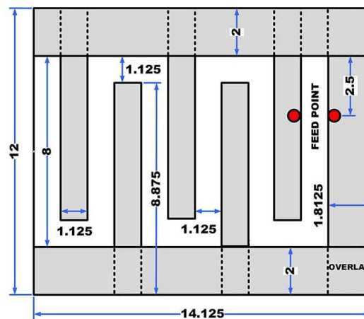
Figure 4: dimensions of 3 in. version of antenna.
